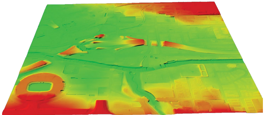
3D elevation data for an area of Denver, Colorado, in the form of a lidar point cloud (top) and a derived bare-earth digital elevation model (bottom). These data along with other products provide valuable productivity, safety, and cost-saving benefits to infrastructure improvement projects.
