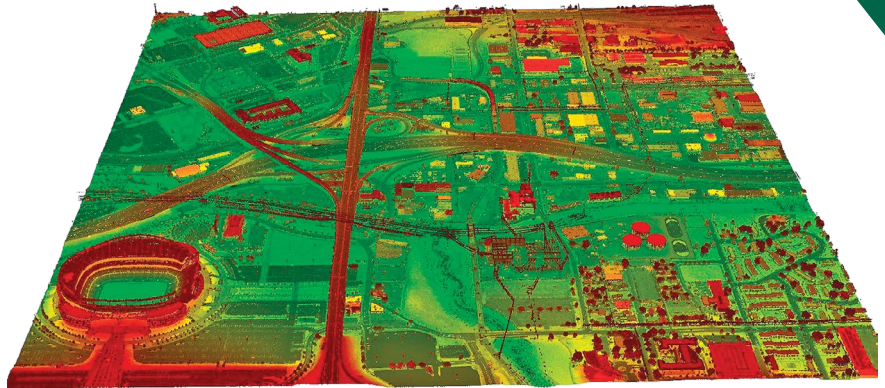
3D elevation data for an area of Denver, Colorado, in the form of a lidar point cloud (top) and a derived bare-earth digital elevation model (bottom). These data along with other products provide valuable productivity, safety, and cost-saving benefits to infrastructure improvement projects.
